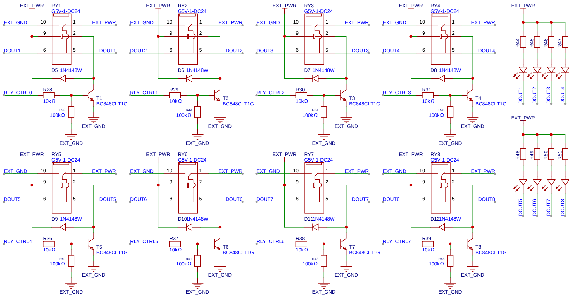
DIGITAL OUTPUT RELAY
